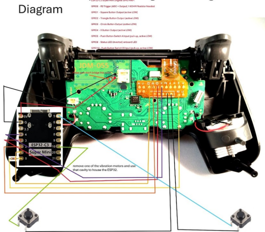
The Future is a Po4 Controller (IOM-648-6000). Wiring is the same as the IOM-655 Super Old Change is the Battery Connector as is illustrated. Here that the only change ESP32-C3 Super Mini Original Wiring ESP32-C3 Super Mini Original GPIO MAP Diagram GPIO0 - RST Trigger (GPIO + Output) 1 LED/HX Resistor needed GPIO1 - Square Wave/Output (Jumper L0W)
